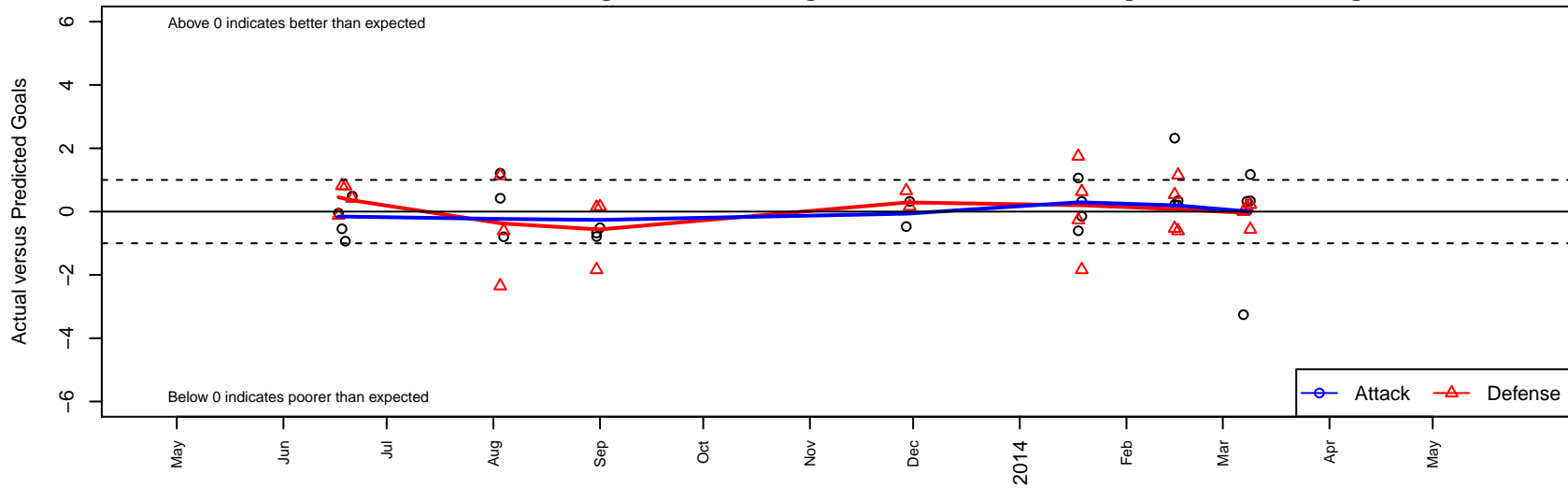
Heat FC 01 RM G00 Dots are actual minus expected GF (blue circles) and GA (red triangles). Blue line is smoothed change in attack strength. Red is smoothed change in defense strength.
